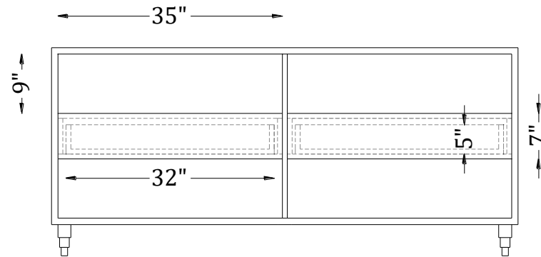
INTERNAL VIEW
